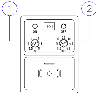
TIMER (Front view)
